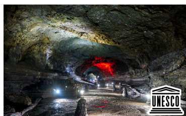
Manjanggul Cave
